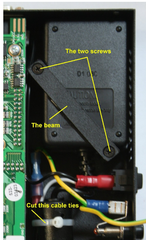
Figure 1: The internal PSU of the programmer
